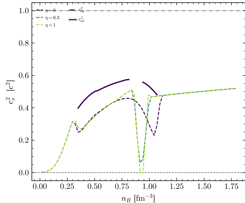
fixed Y_C = 0.1 , T = 0 MeV
