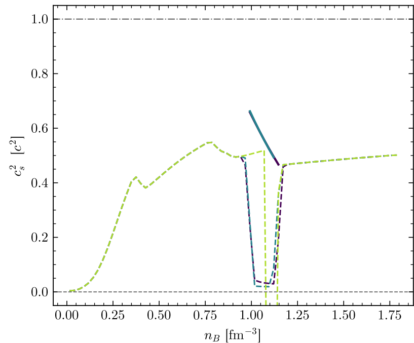
fixed Y_C = 0.4 , T = 0.1 MeV
