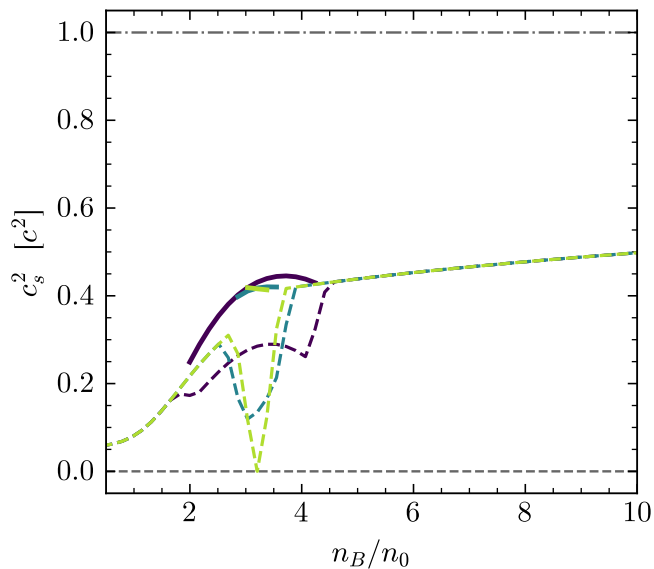
Y_C = 0.4 , T = 0.1 MeV
