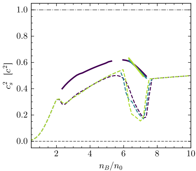
Y_C = 0.1 , T = 0 MeV
