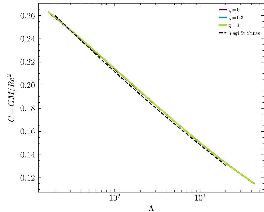
binary Love, \mathcal{M}_c = 1.186 M_\odot
