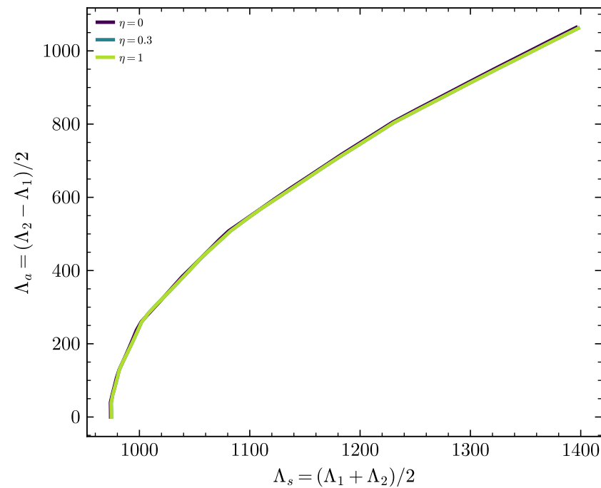
binary Love, \mathcal{M}_c = 1.186 M_\odot
