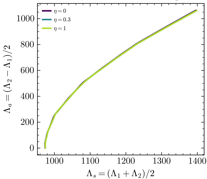
binary Love, \mathcal{M}_c = 1.186 M_\odot
