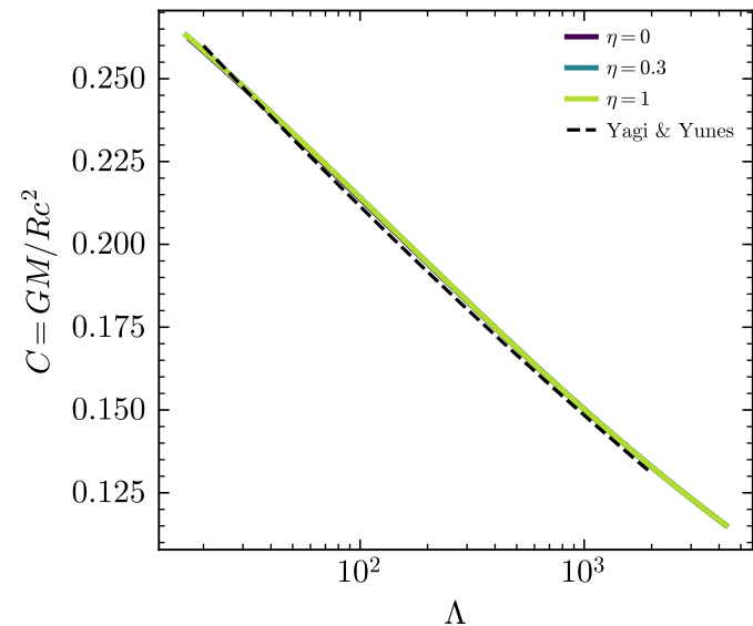
binary Love, \mathcal{M}_c = 1.186 M_\odot
