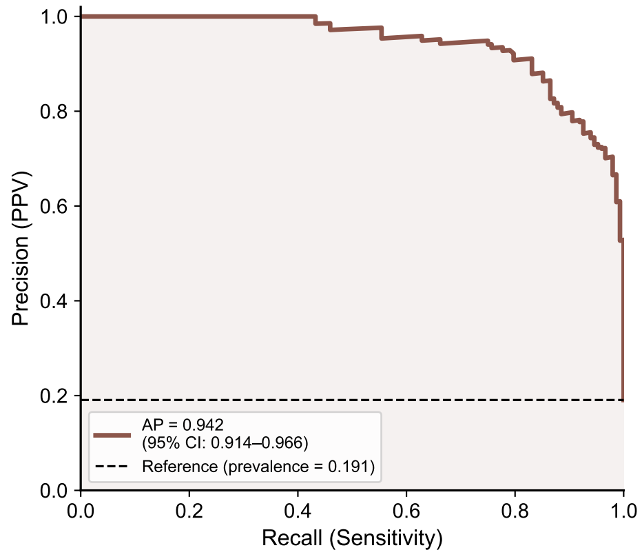
Precision-Recall Curve
