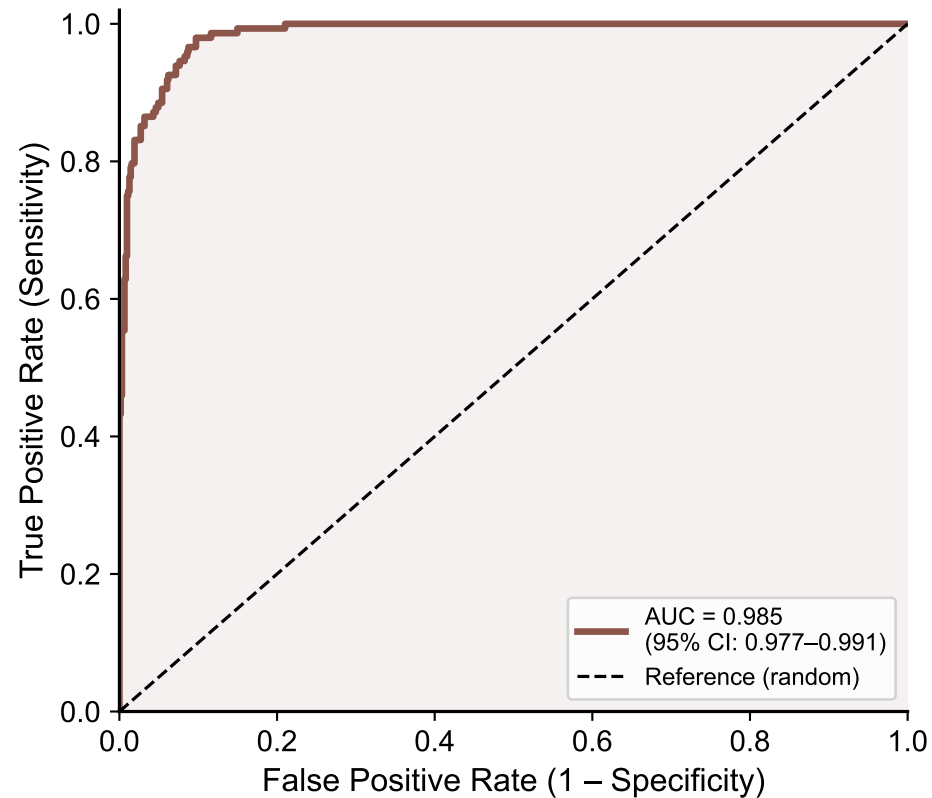
ROC Curve
