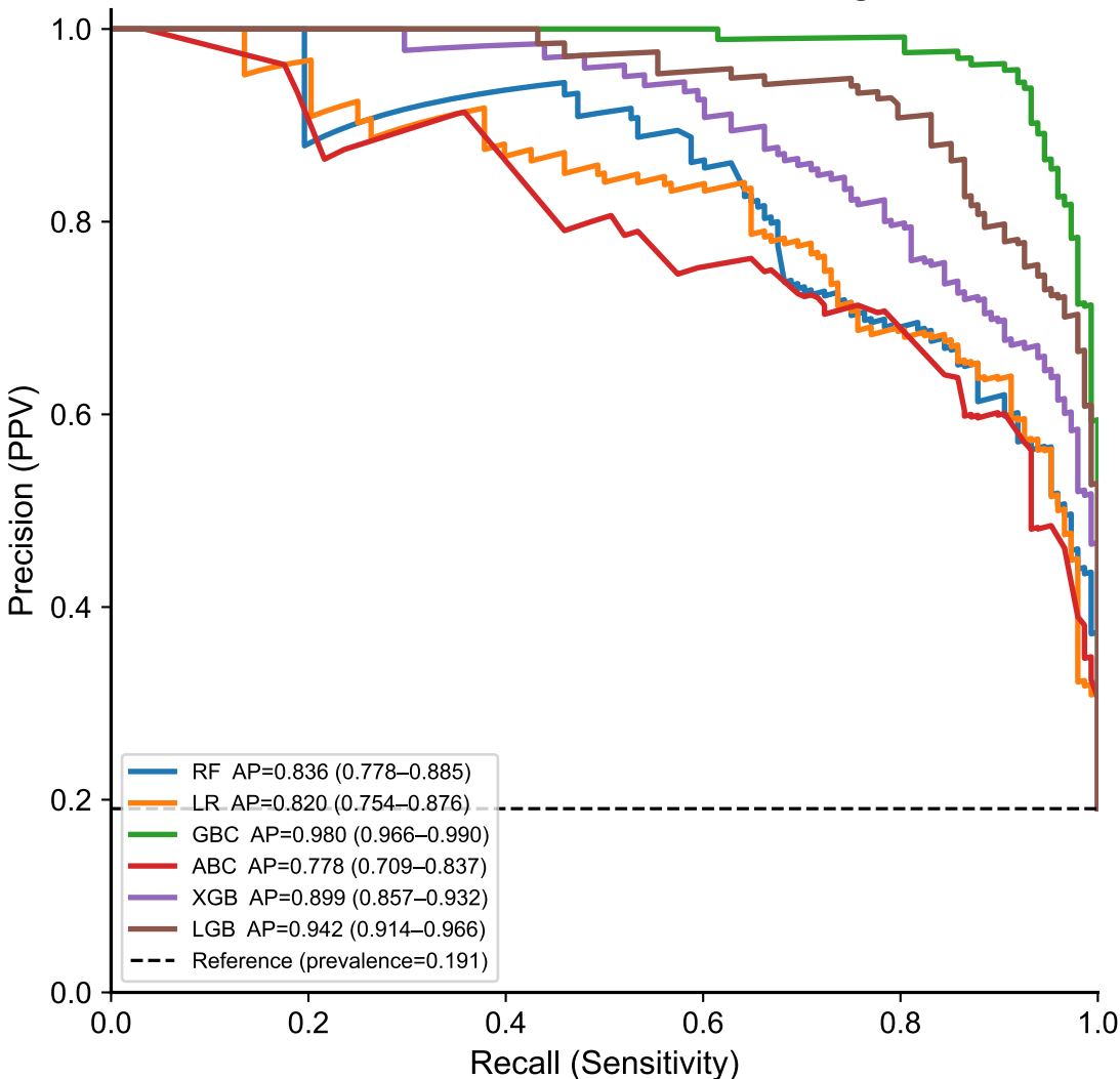
Precision-Recall Curves — Training Set
