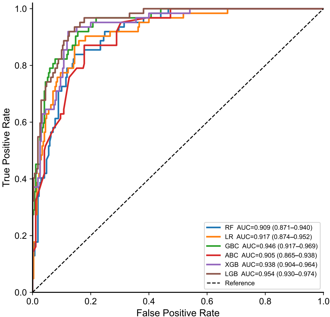
ROC Curves — Internal Validation
