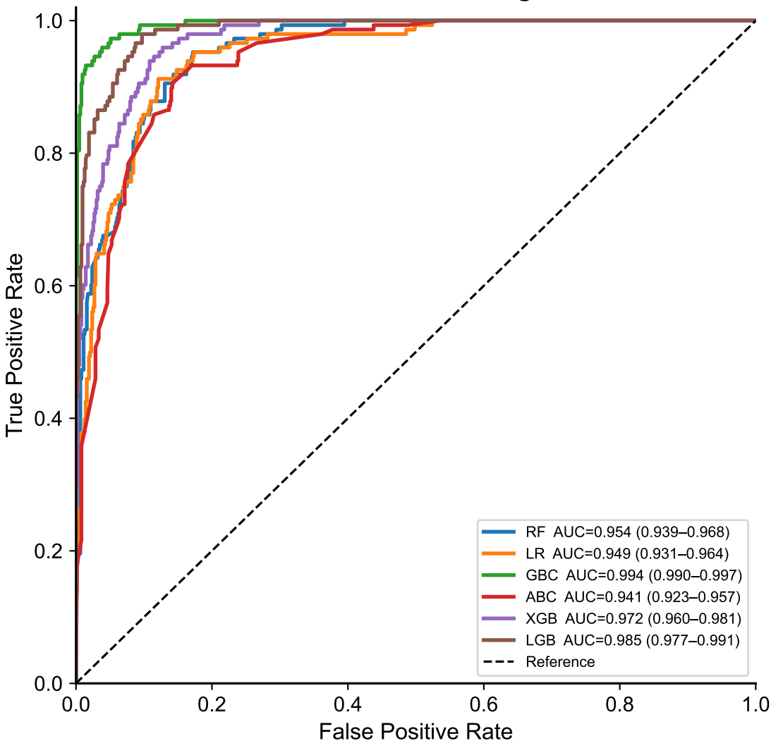
ROC Curves — Training Set
