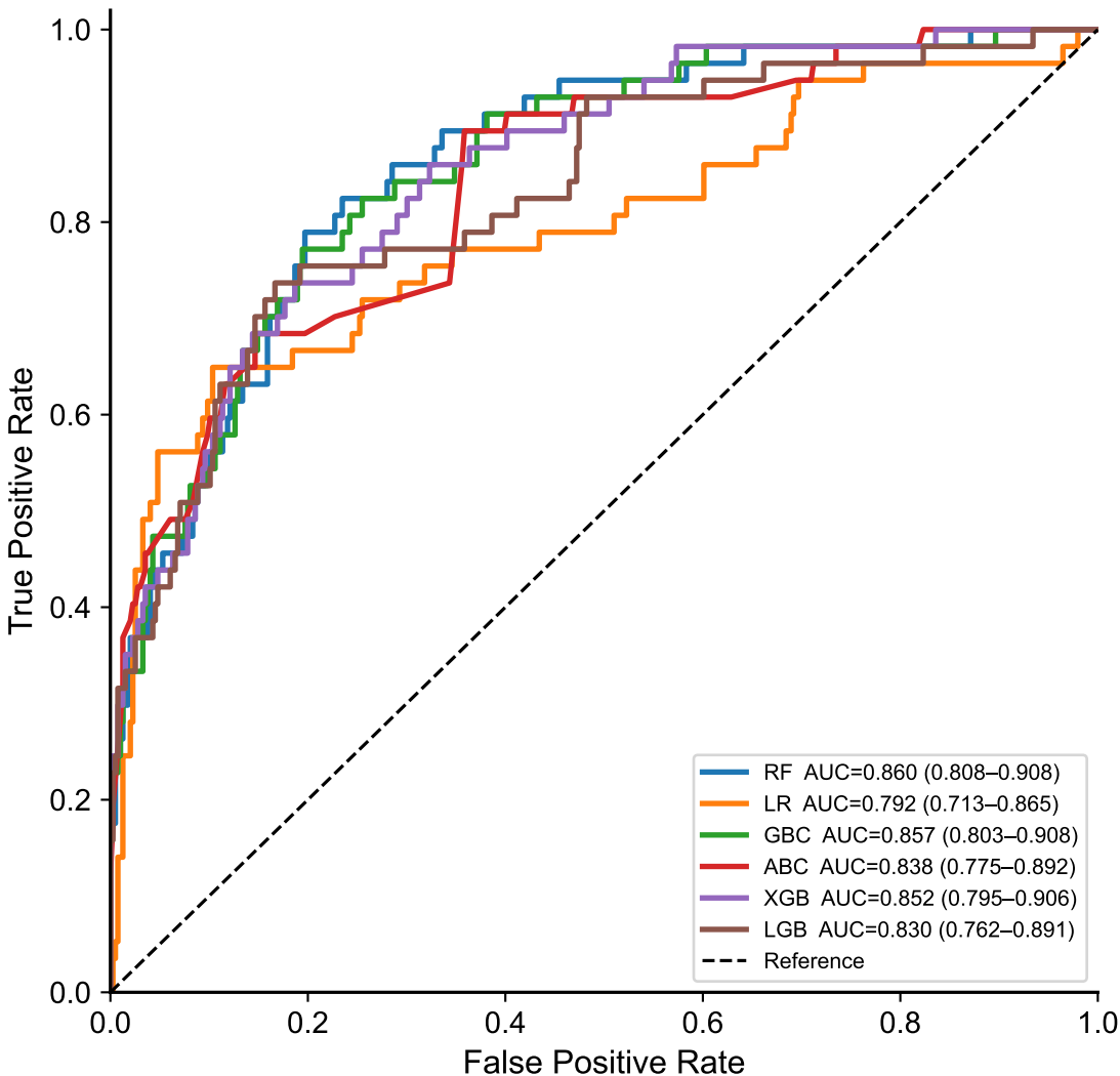
ROC Curves — External Validation
