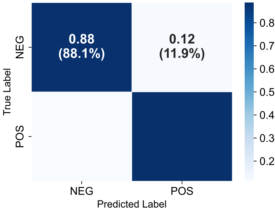
LGB — Internal Validation (Normalized)
