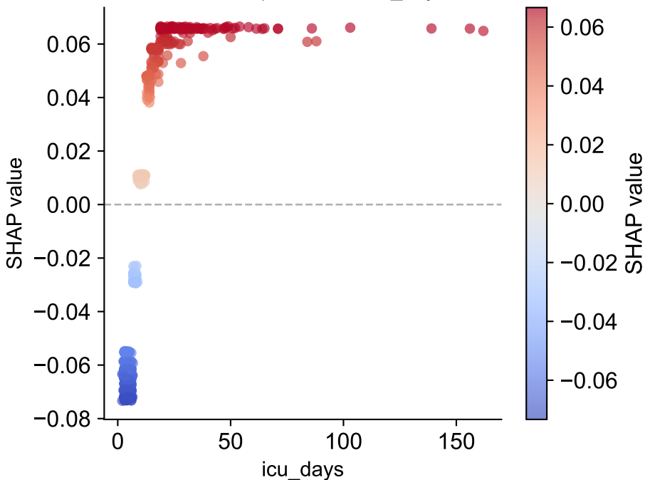
ABC — Dependence: icu_days
