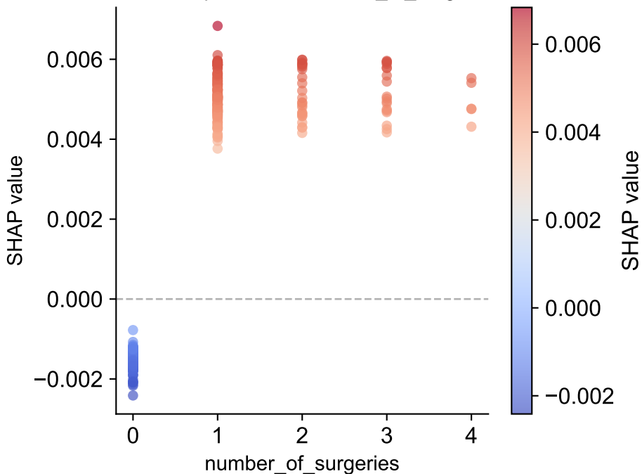
ABC — Dependence: number_of_surgeries
