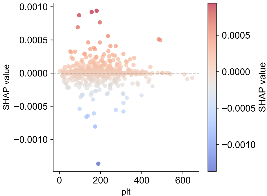
ABC — Dependence: plt
