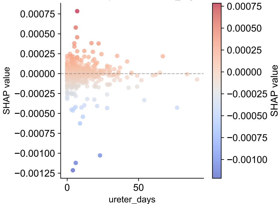
ABC — Dependence: ureter_days
