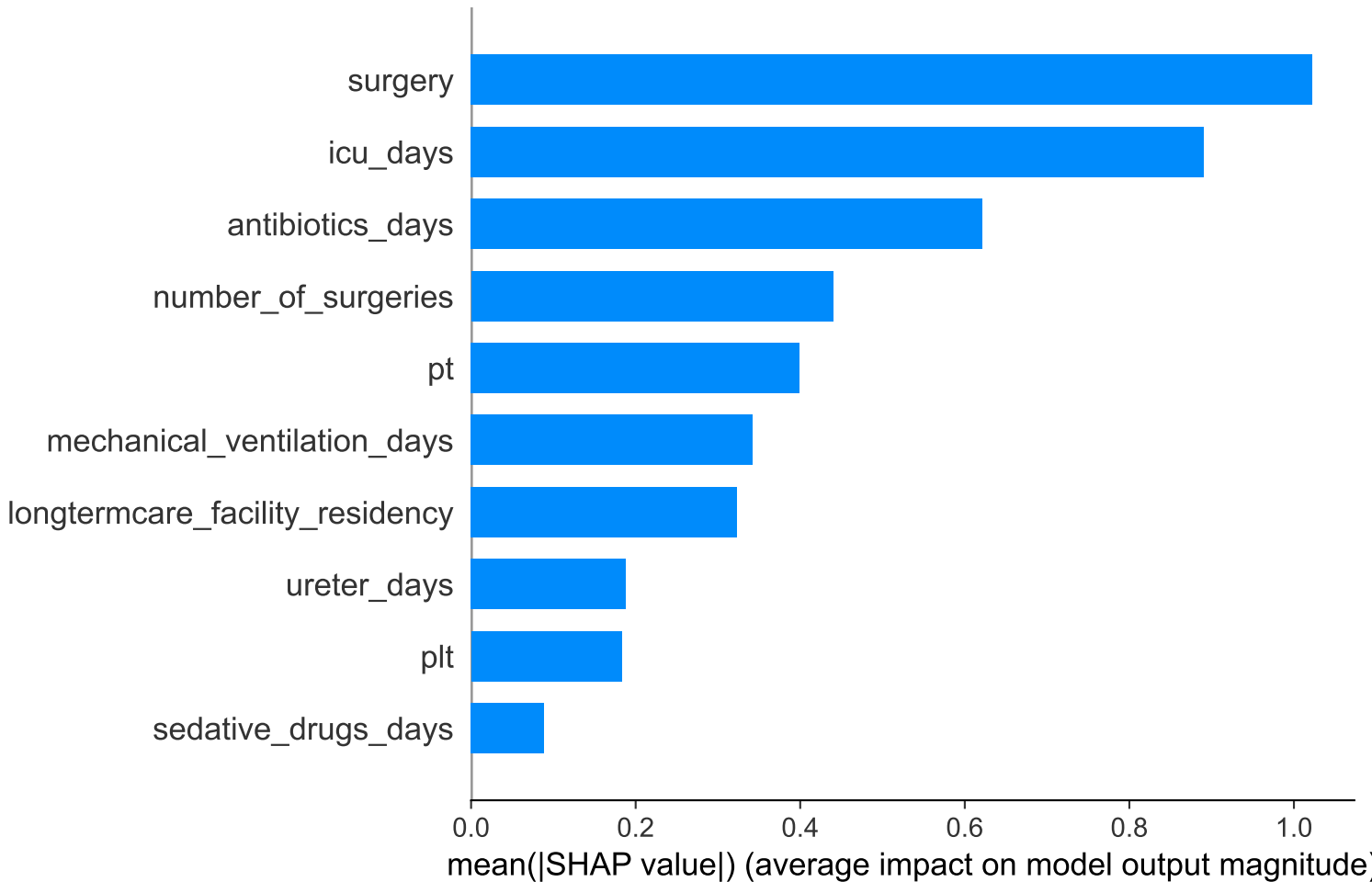
GBC — Mean |SHAP| Feature Importance
