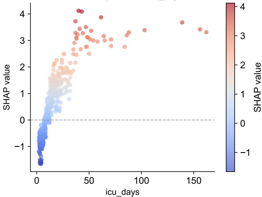
GBC — Dependence: icu_days
