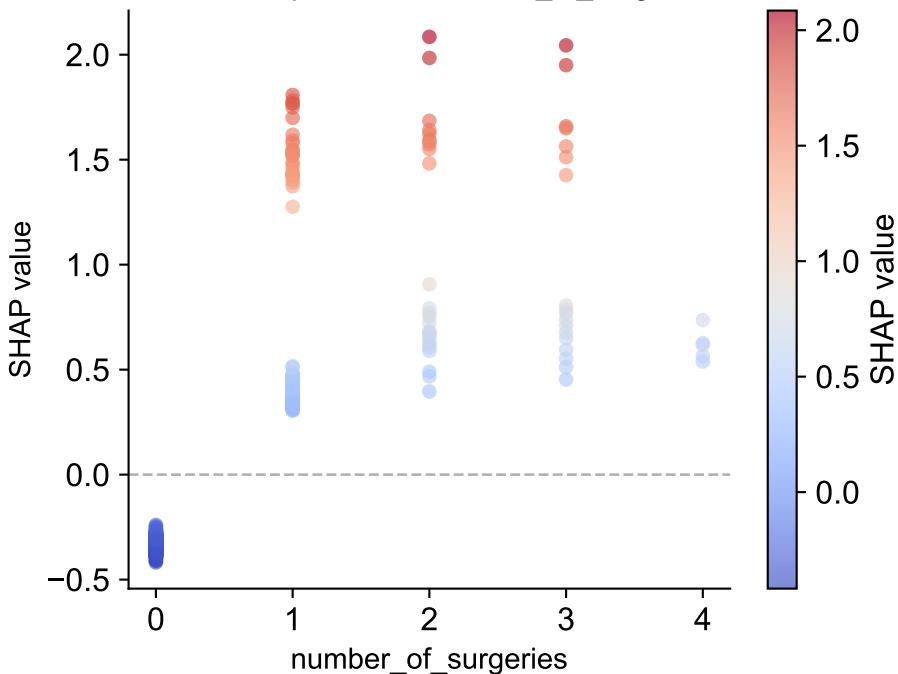
GBC — Dependence: number_of_surgeries
