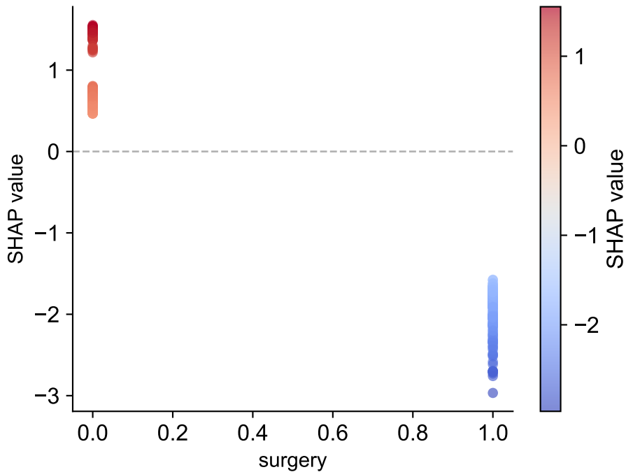
GBC — Dependence: surgery
