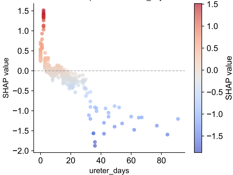
GBC — Dependence: ureter_days
