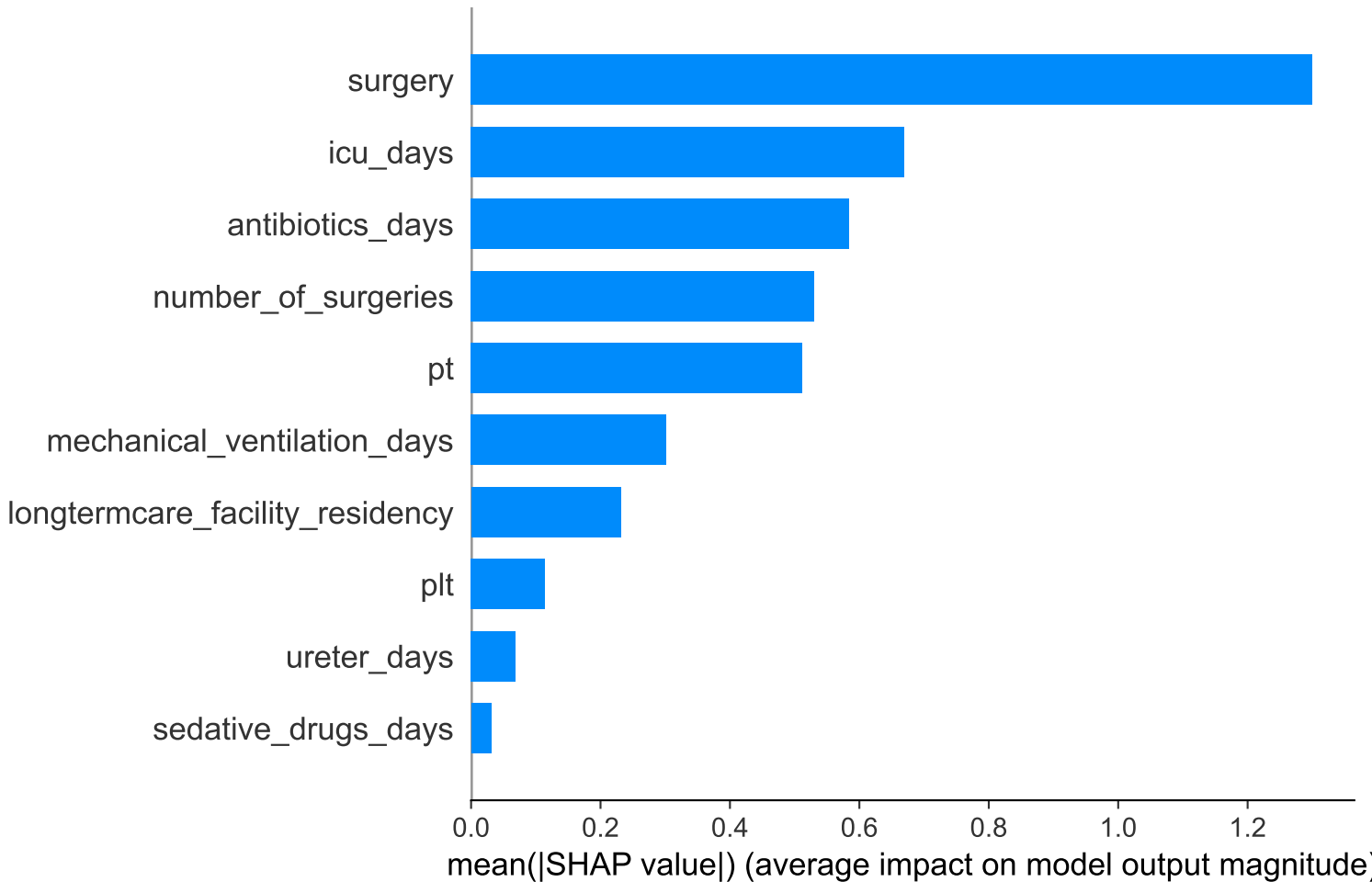
LGB — Mean |SHAP| Feature Importance
