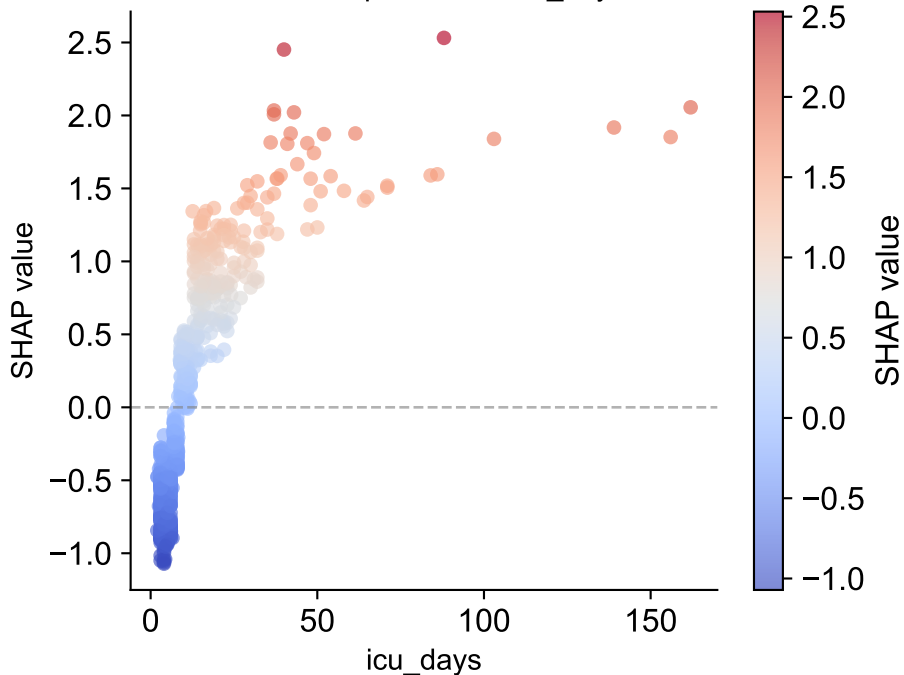
LGB — Dependence: icu_days
