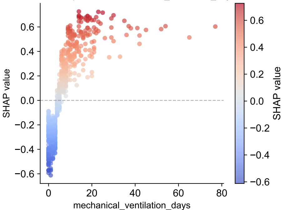
LGB — Dependence: mechanical_ventilation_days
