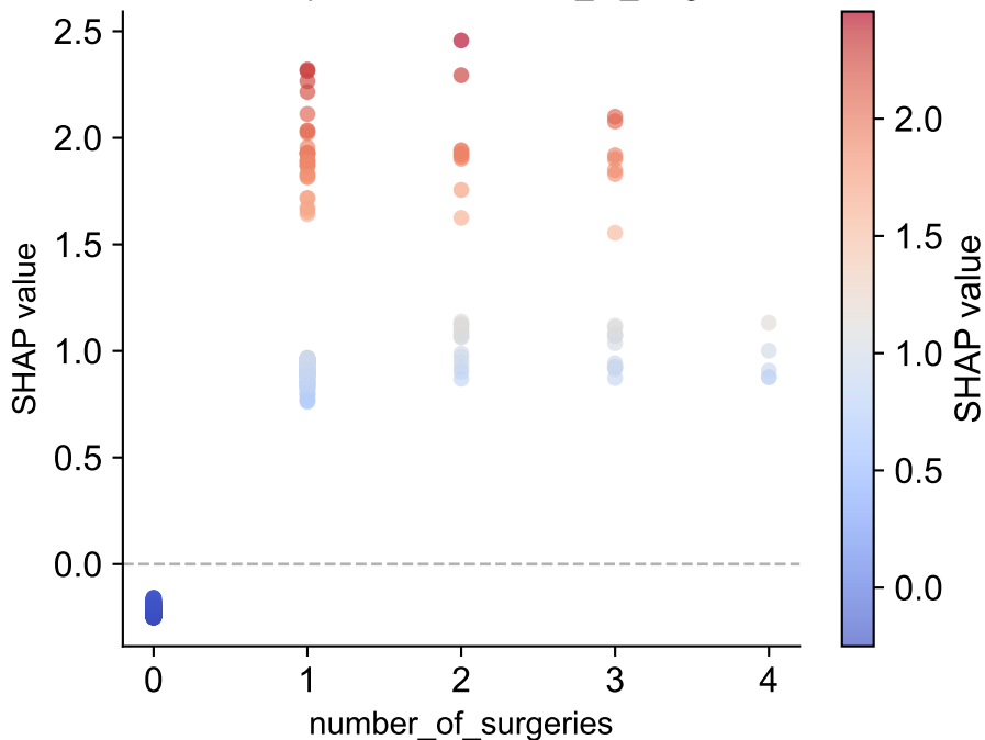
LGB — Dependence: number_of_surgeries
