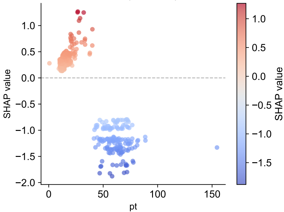
LGB — Dependence: pt
