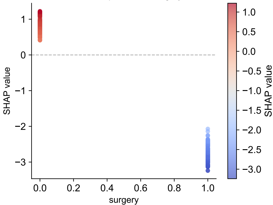
LGB — Dependence: surgery
