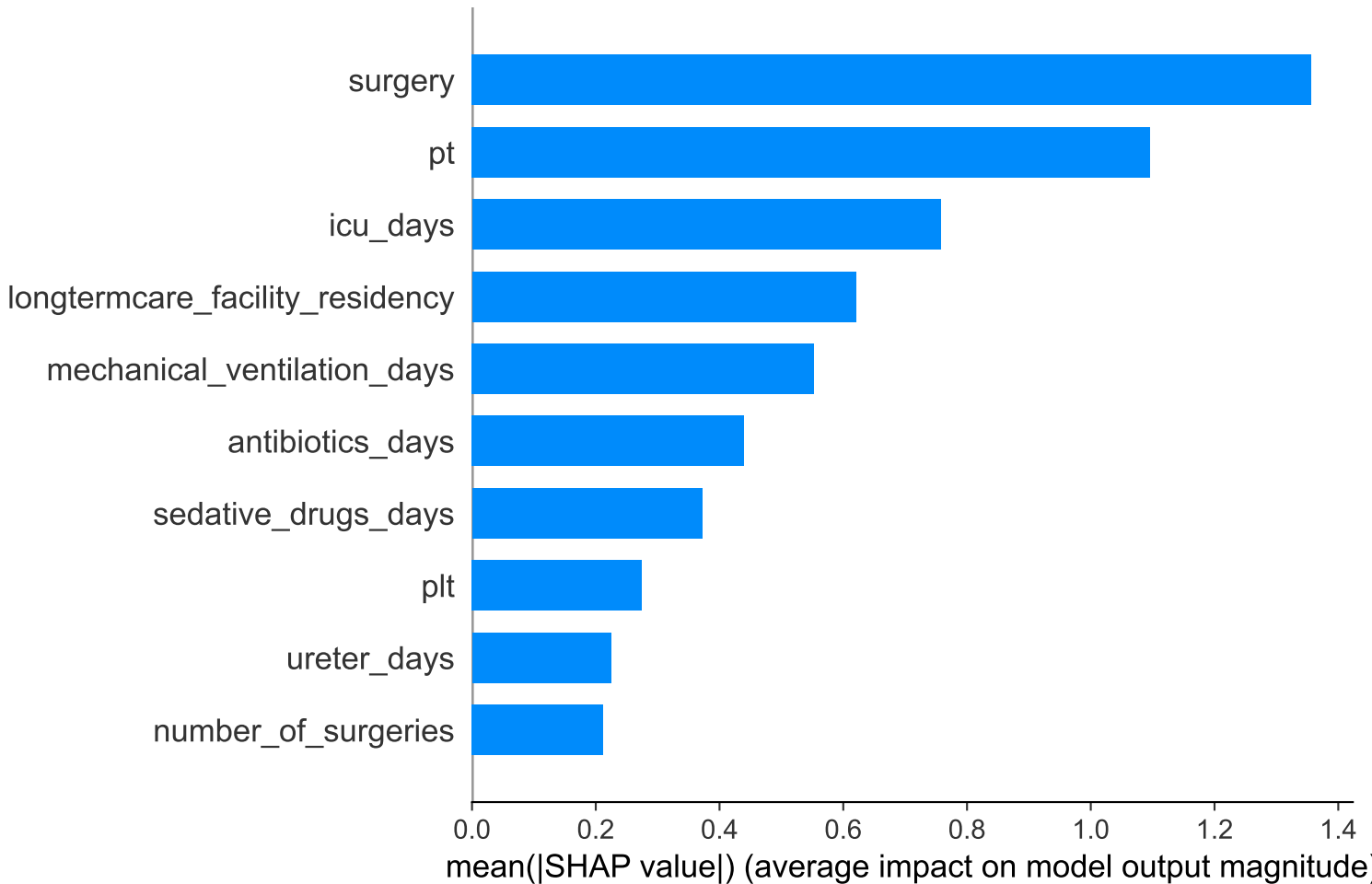
LR — Mean |SHAP| Feature Importance
