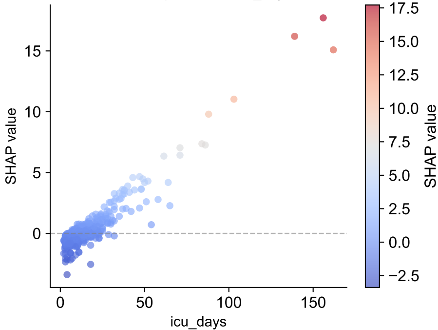
LR — Dependence: icu_days
