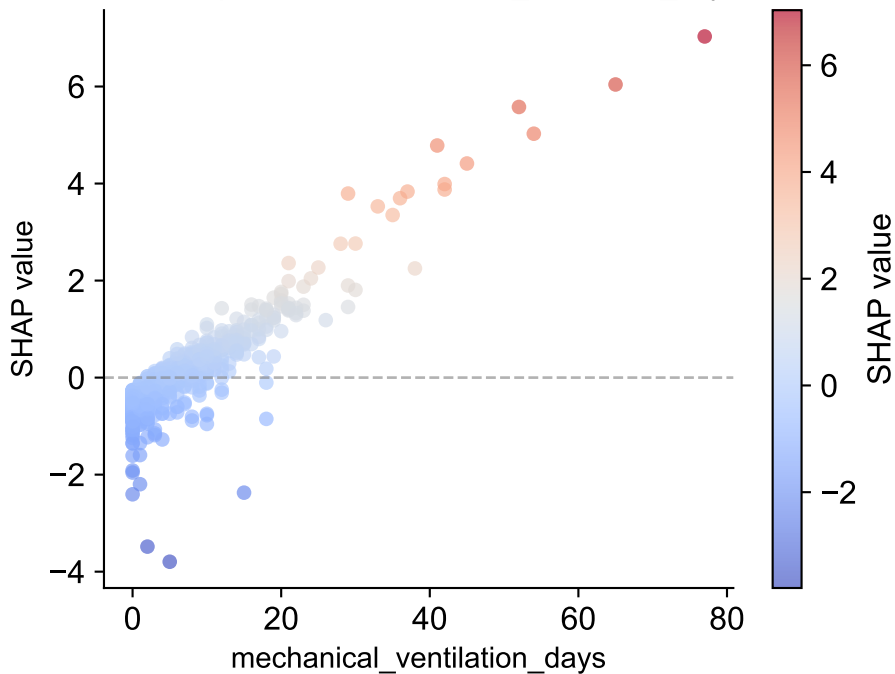
LR — Dependence: mechanical_ventilation_days
