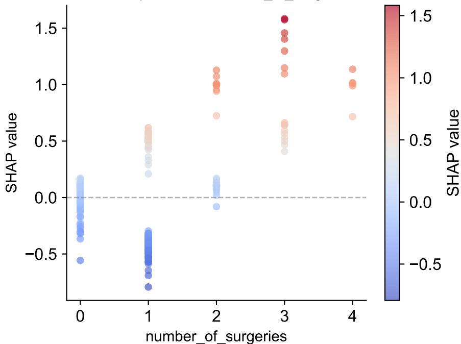
LR — Dependence: number_of_surgeries
