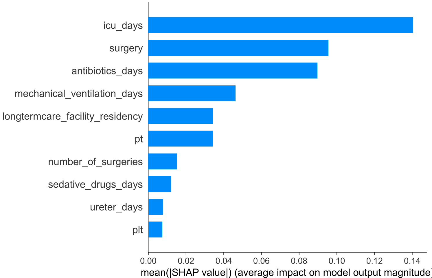
RF — Mean |SHAP| Feature Importance
