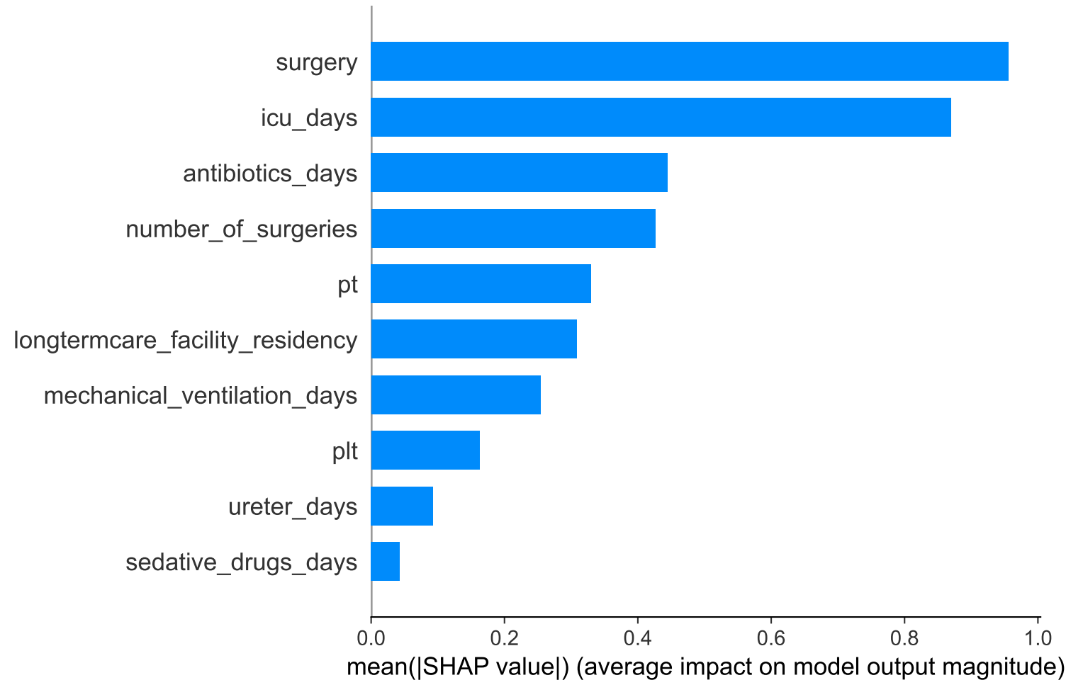
XGB — Mean |SHAP| Feature Importance
