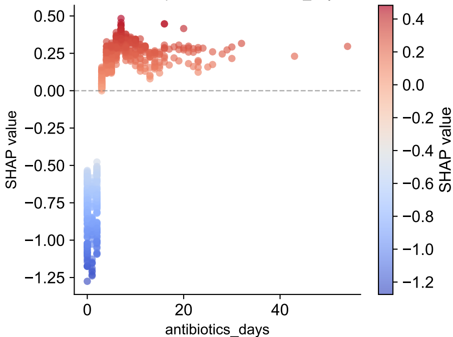
XGB — Dependence: antibiotics_days
