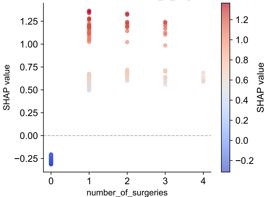
XGB — Dependence: number_of_surgeries
