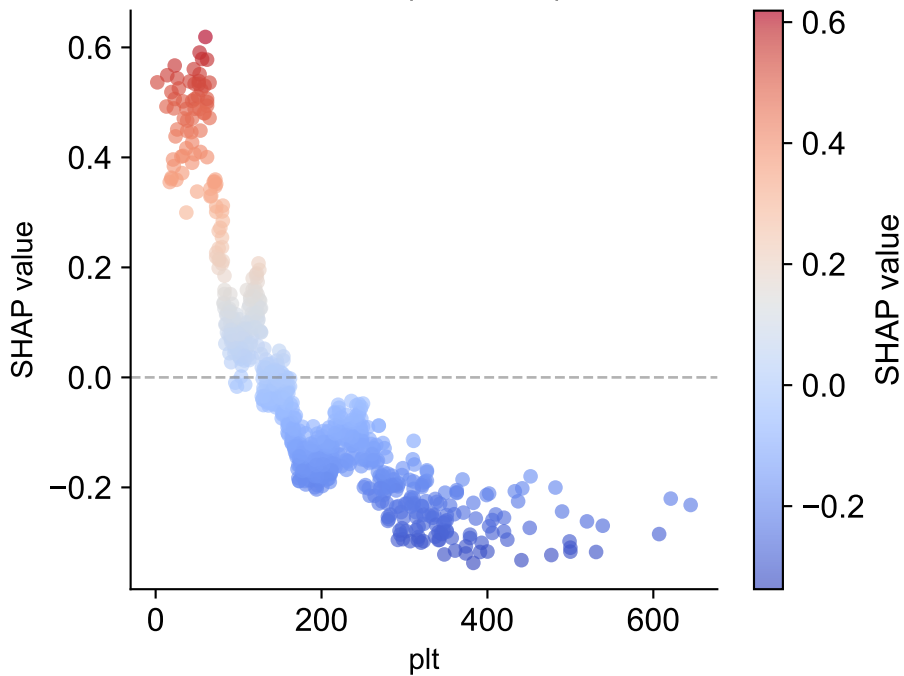
XGB — Dependence: plt
