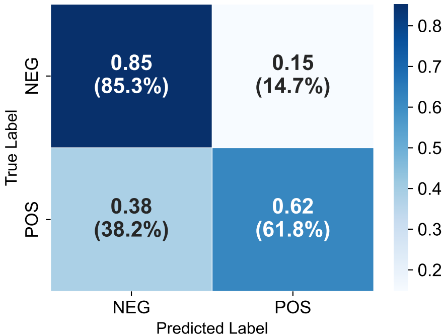
RF — External Validation (Normalized)
