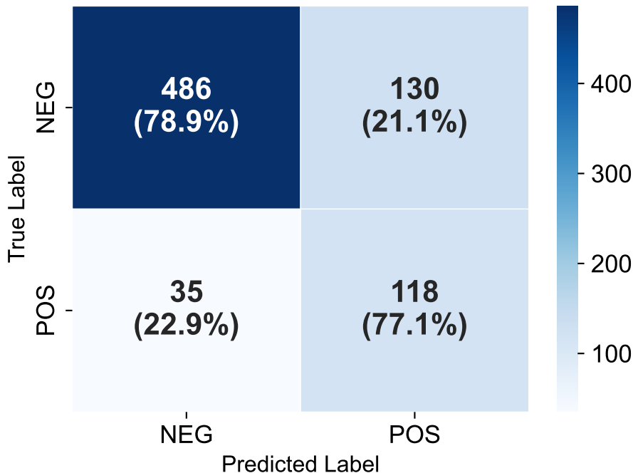
RF — Training Set
