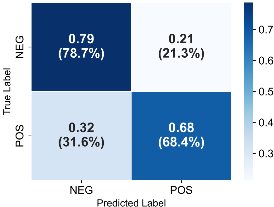
RF — Internal Validation (Normalized)
