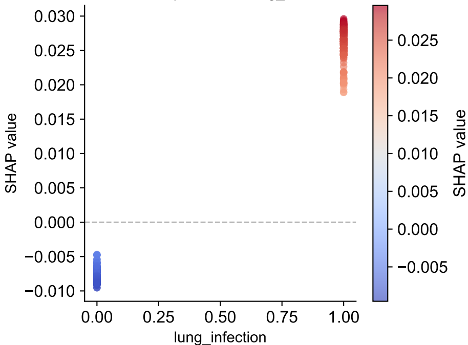
ABC — Dependence: lung_infection
