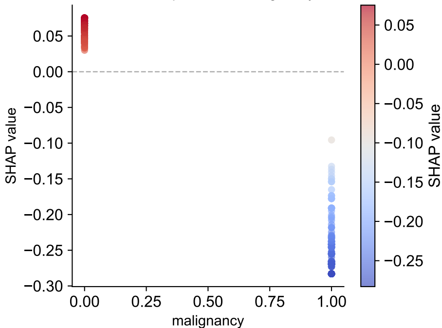
GBC — Dependence: malignancy
