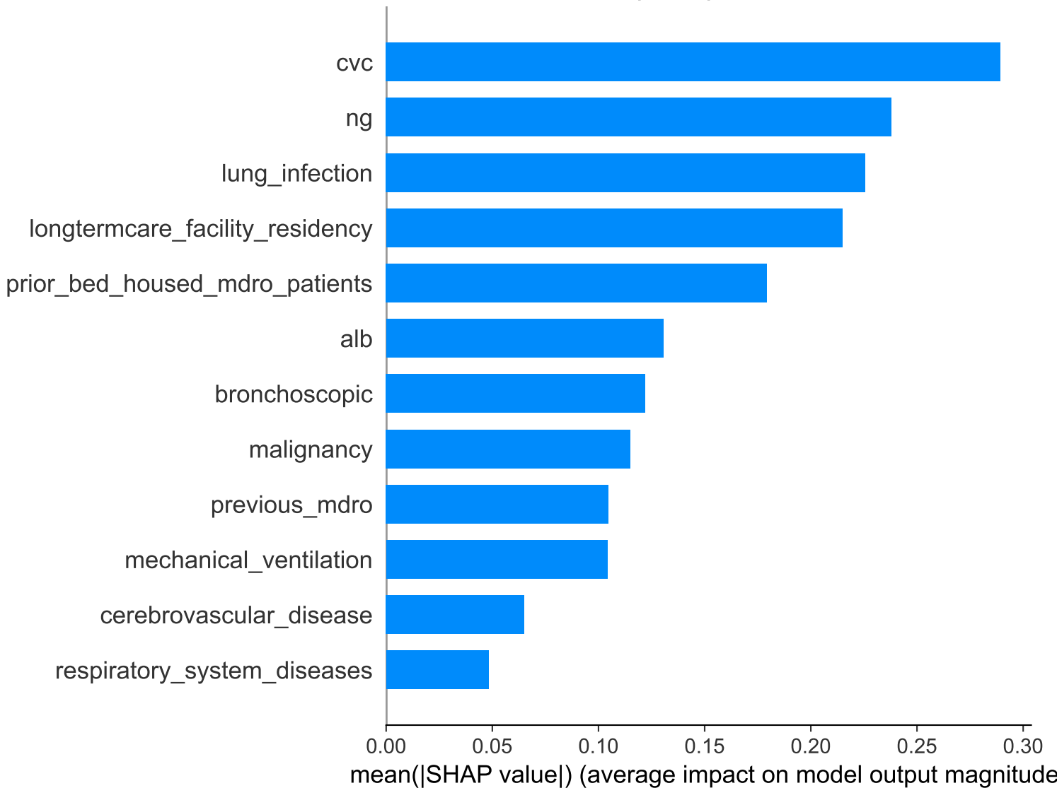
LGB — Mean |SHAP| Feature Importance
