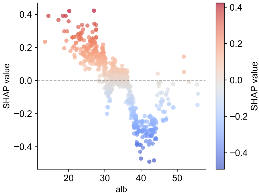
LGB — Dependence: alb
