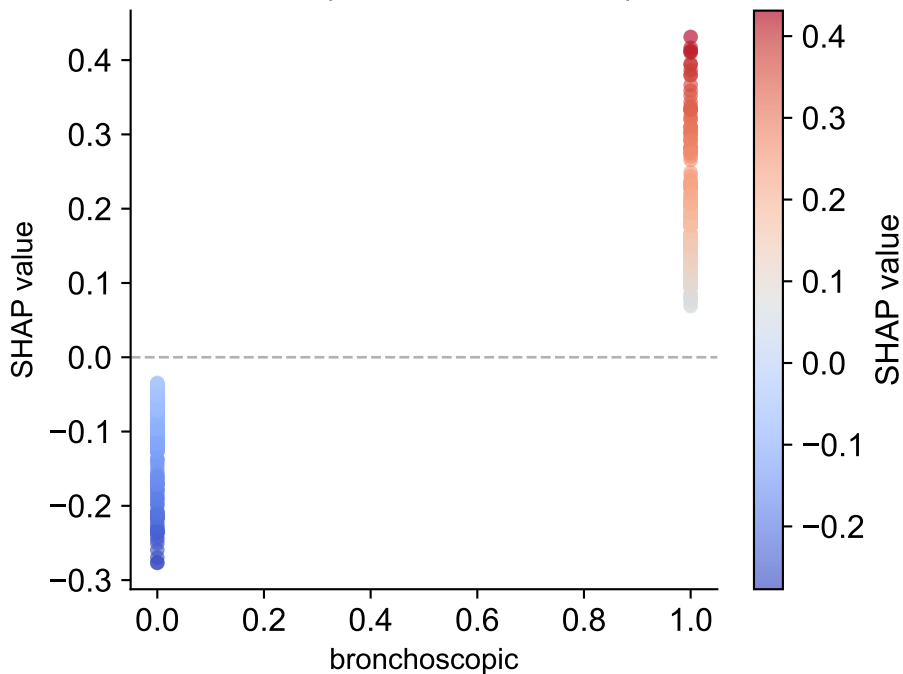
LGB — Dependence: bronchoscopic
