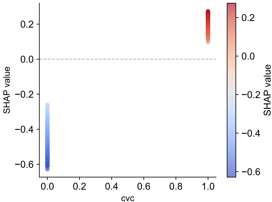
LGB — Dependence: cvc
