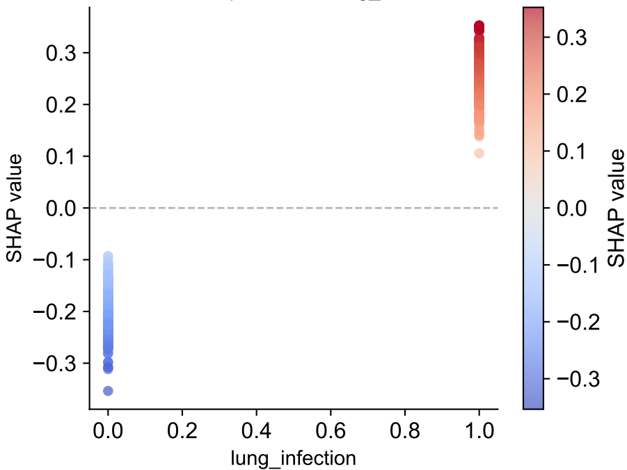
LGB — Dependence: lung_infection
