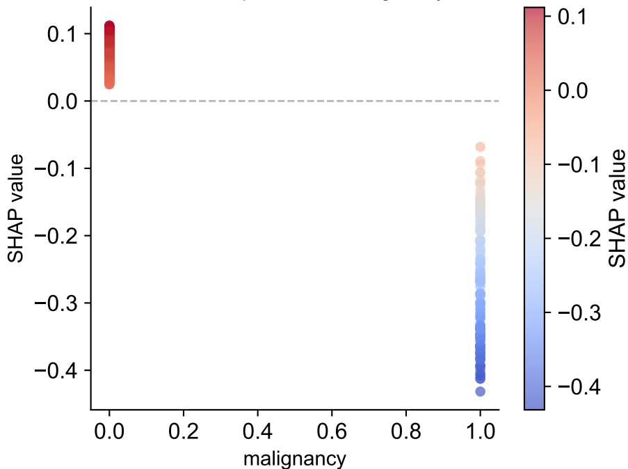
LGB — Dependence: malignancy
