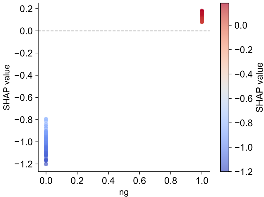
LGB — Dependence: ng
