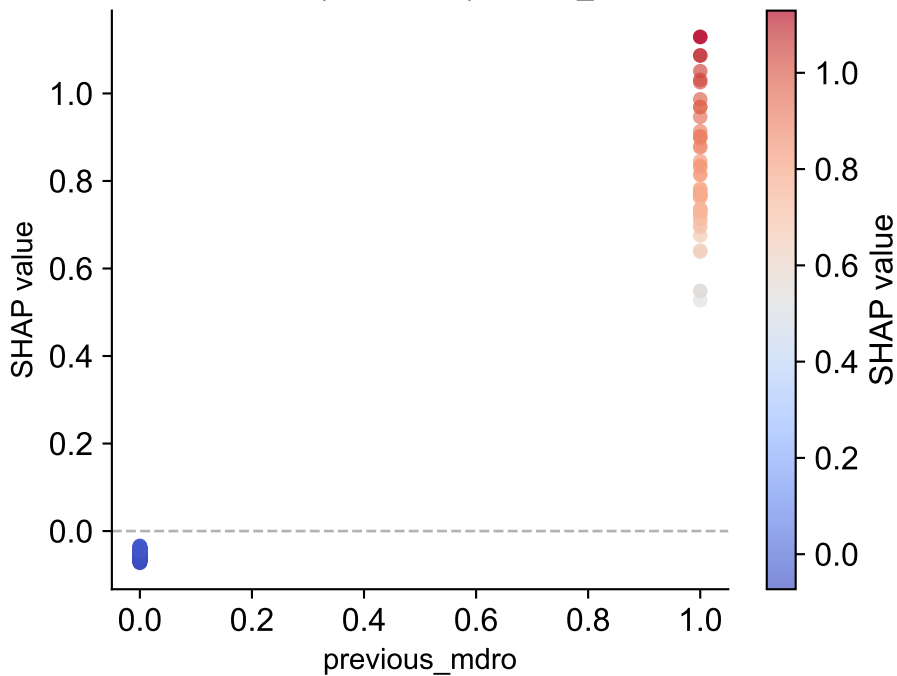
LGB — Dependence: previous_mdرو
