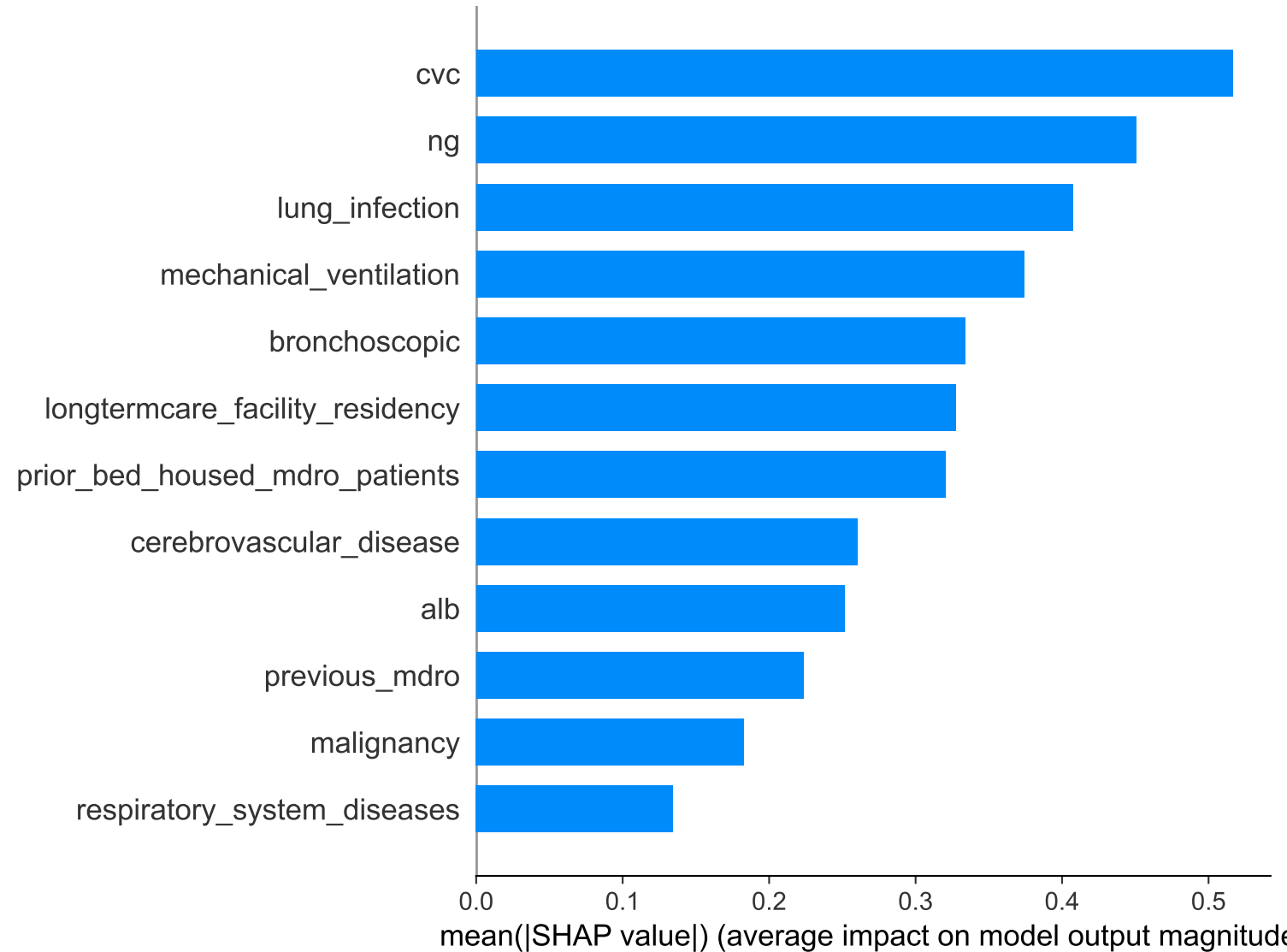
LR — Mean |SHAP| Feature Importance
