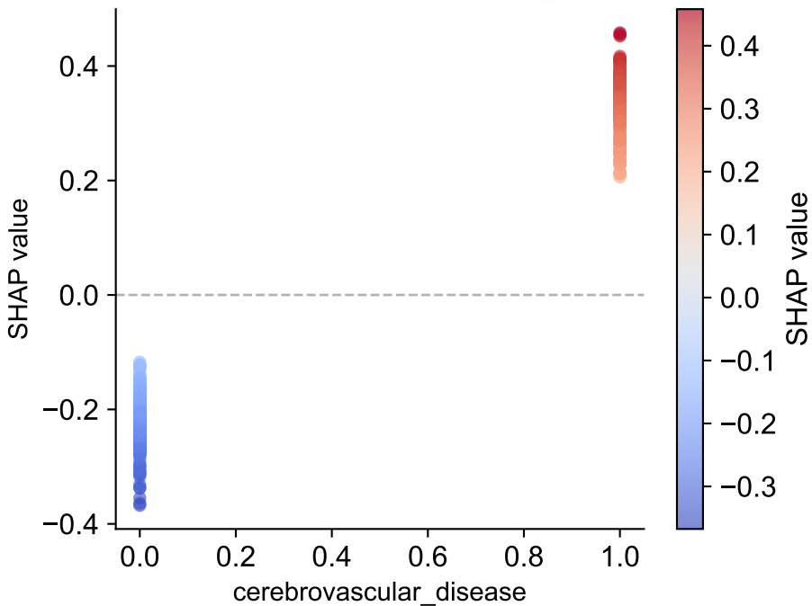
LR — Dependence: cerebrovascular_disease
