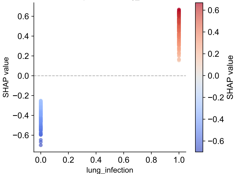
LR — Dependence: lung_infection
