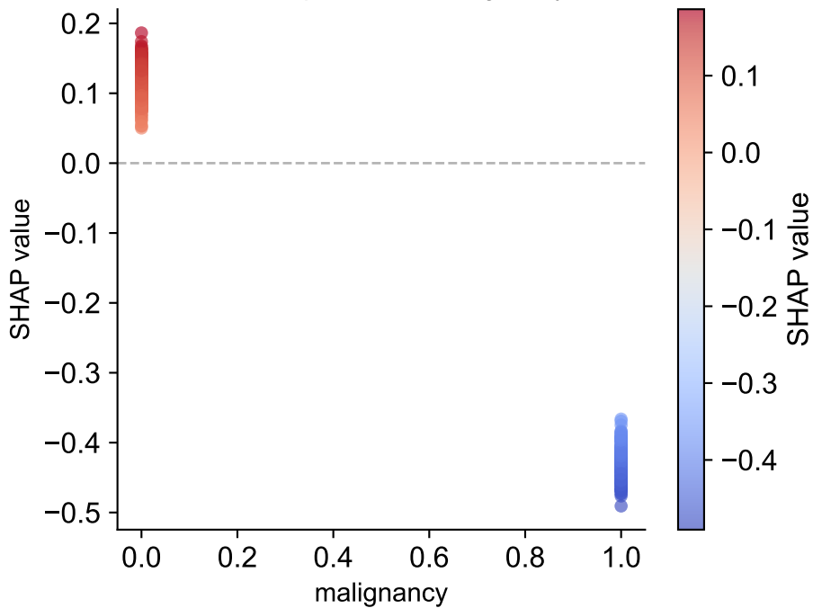
LR — Dependence: malignancy
