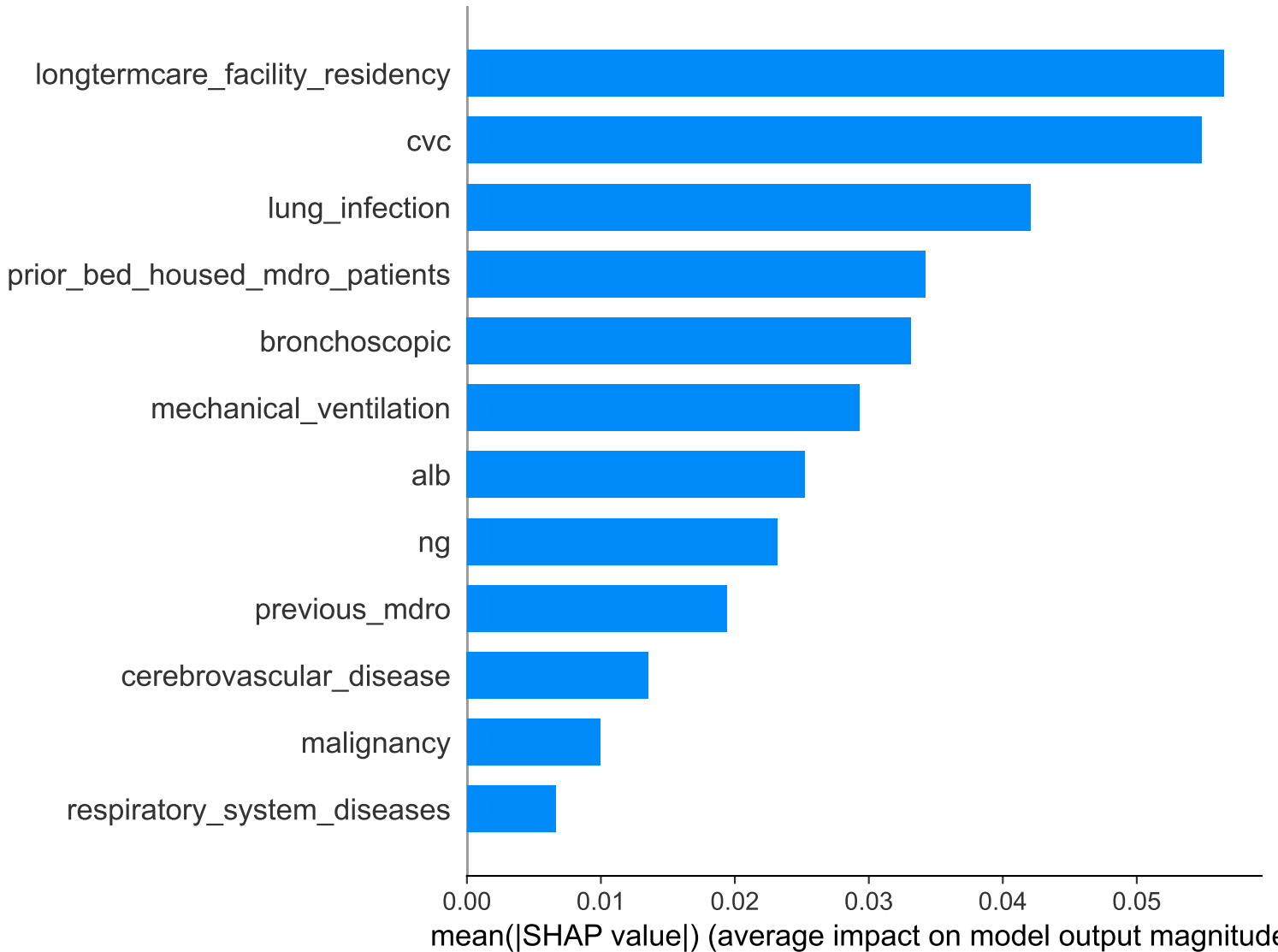
RF — Mean |SHAP| Feature Importance
